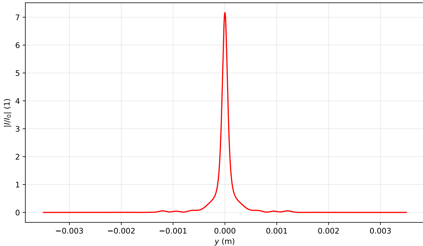
Intensity profile I(x=0, y, z=1.433)/I_0 , \text{Pin}=5.5\text{Pcr} , artificial time
